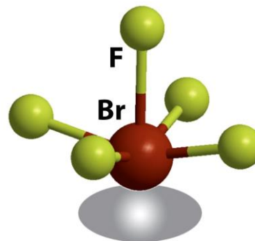
4 BrF 5 , C 4v
